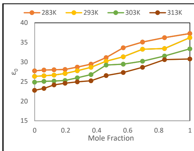
Fig.1. Variation of static dielectric constant ( \epsilon_0 ) as a function of mole fraction
