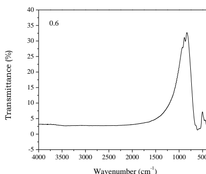
Fig.4 (c): IR spectra of Y_3In_xFe_{5-x}O_{12} of typical samples x = 0.6 .
