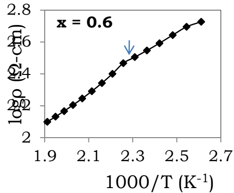
Fig. 5 : Variation of \log \rho versus 1000/T of Y_3In_xFe_{5-x}O_{12} . ( x = 0.0, 0.2 and 0.6 ).
