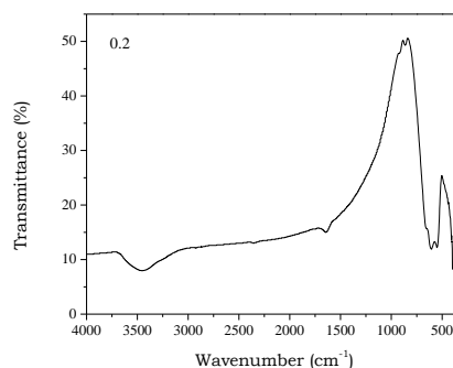
Fig.4 (b): IR spectra of Y_3In_xFe_{5-x}O_{12} of typical sample x = 0.2 .
