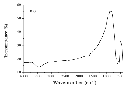
Fig.4 (a): IR spectra of Y_3In_xFe_{5-x}O_{12} of typical sample x = 0.0 .
